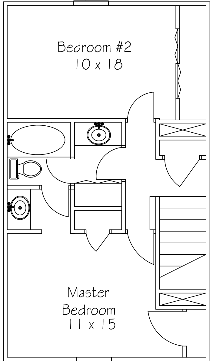
Unit B Floorplan Second Floor
